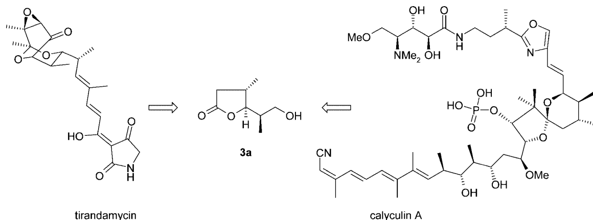
Scheme 2. Lactone 3a as a key intermediate for the synthesis of tirandamycin and calyculin A
