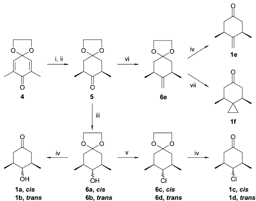
Scheme 3. (i) H_2 , Pd/C, 5 bar; (ii) Na/MeOH, room temp., 69% (overall); (iii) NaBH_4 , dry MeOH, 0 °C, 90%; (iv) 1% H_2SO_4 /acetone, (1:1), room temp. to 40 °C, 88–92%; (v) PPh_3 , NCS, THF, 61–80%; (vi) MePPh_3^+Br^- , BuLi, dry THF, 91%; (vii) ZnEt_2 , CH_2I_2 , CF_3COOH , CH_2Cl_2 , 0 °C, then 2 N HCl, room temp., 50% (overall)
