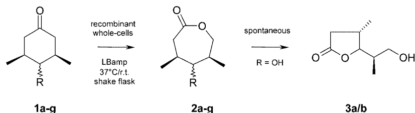
Scheme 1. Biotransformation of functionalized cyclohexanone systems with CHMO-expressing recombinant cells
